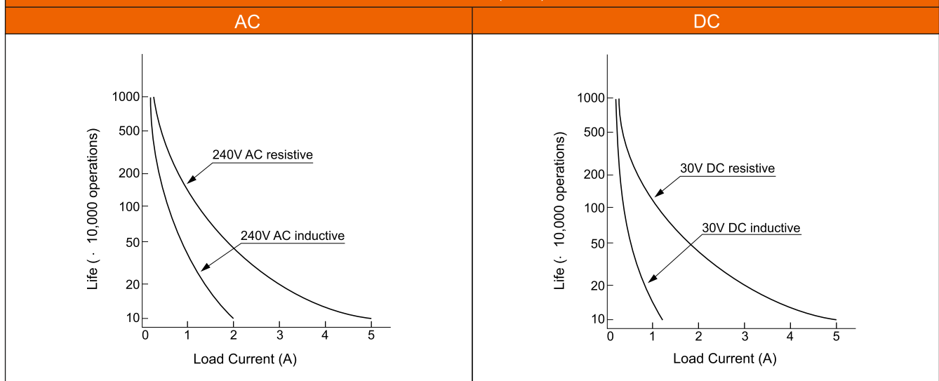
21.14 & 21.24 (4PDT)
